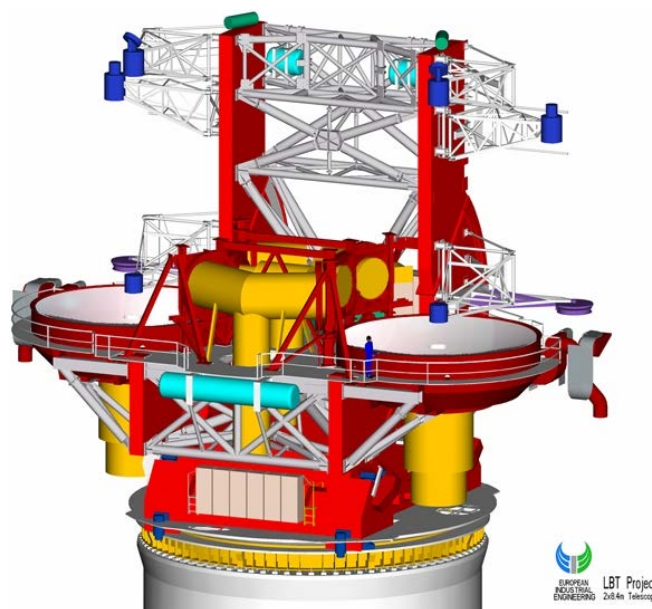
Fig.1: 3d-model of the LBT
