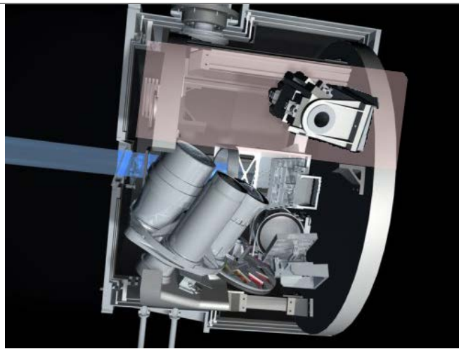
Fig.2: Cut through the LUCI cryostat. The pink area indicates the location of the MOS-unit.
